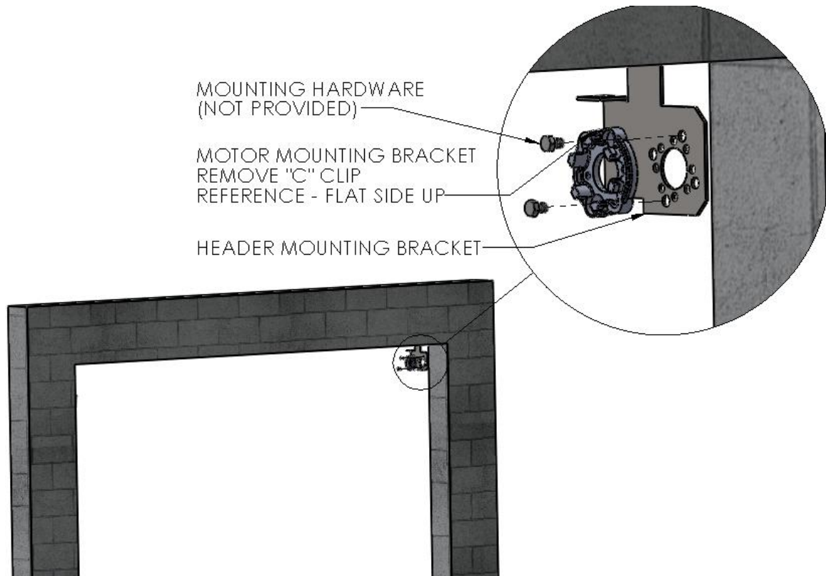
Figure 5 MOUNT MOTOR & HEADER BRACKETS
