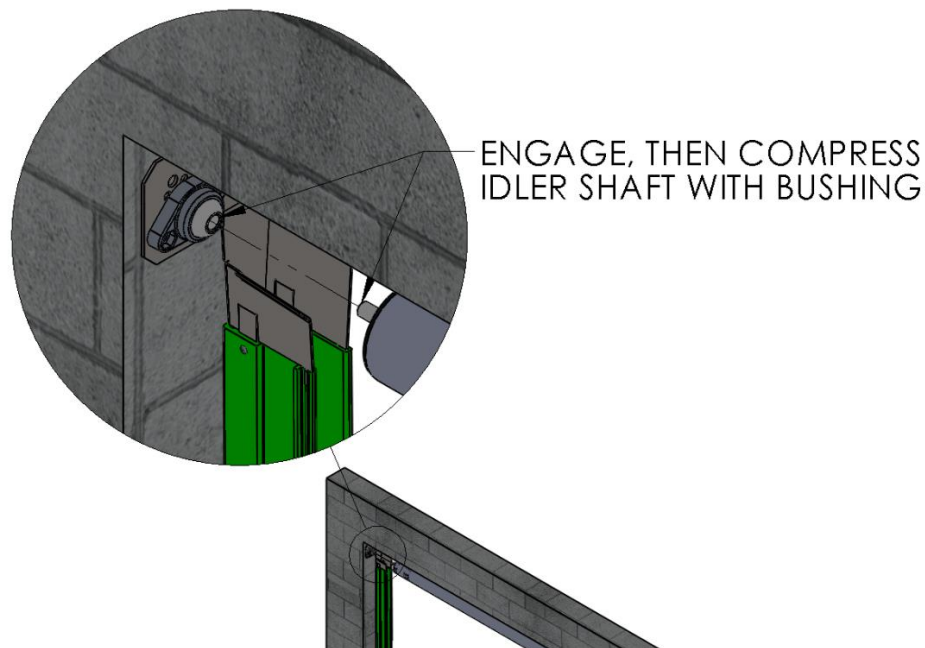
Figure 6 INSTALL L.H. SIDE OF HEADER ASSEMBLY
