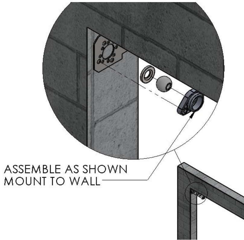
Figure 3 INSTALL HEADER BRACKET AND IDLER ASSEMBLY
