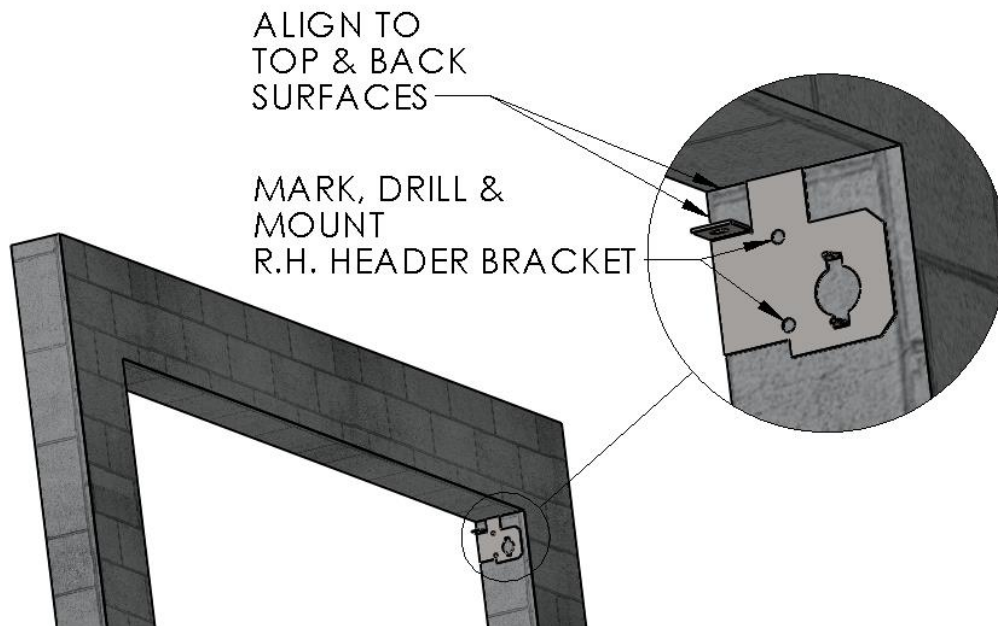
Figure 4 MARK, DRILL, INSTALL R.H. HEADER MOUNTING BRACKET
