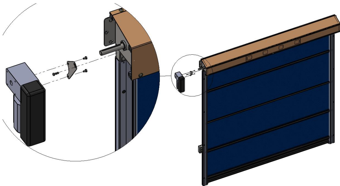
Figure 8 OPERATOR/BRACKET ARRANGEMENT
